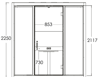
Fixed Center Table with Back Panel
